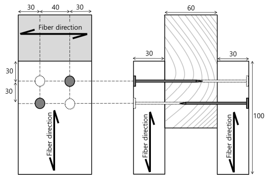
Fig. 1. Specimens for evaluating a nail lateral resistance (unit: mm).
